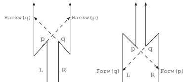
Fig. 1. Deadlocks
