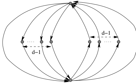
Fig. 4. Planar digraph of maximum out-degree degree d \geq 41 and diameter 2, having precisely 2d vertices
