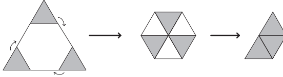
Fig. 3. A flat 3-folding of an equilateral triangle to a trapezoid
