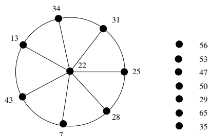
Fig. 8. Exclusive sum labeling of wheel W_7
