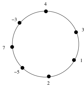
Fig. 7. Integral sum labeling of C_7
