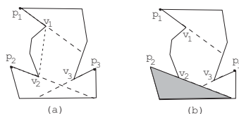
Fig. 2. A polygon satisfying the condition C1
