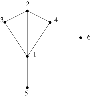
Fig. 11. Sum labeling of bill graph B_6
