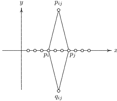
Fig. 3. Constructing a unit-distance spanning subgraph of K_{m,n}
