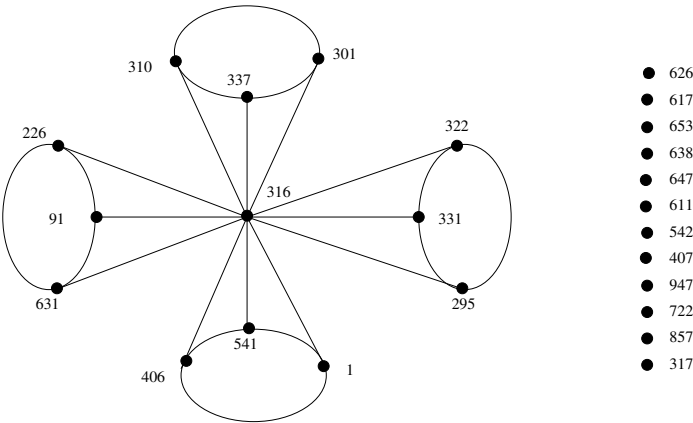
Fig. 10. Exclusive sum labeling of multicone (M_4^3)
